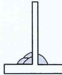
MACROETCH TEST SPECIMEN
