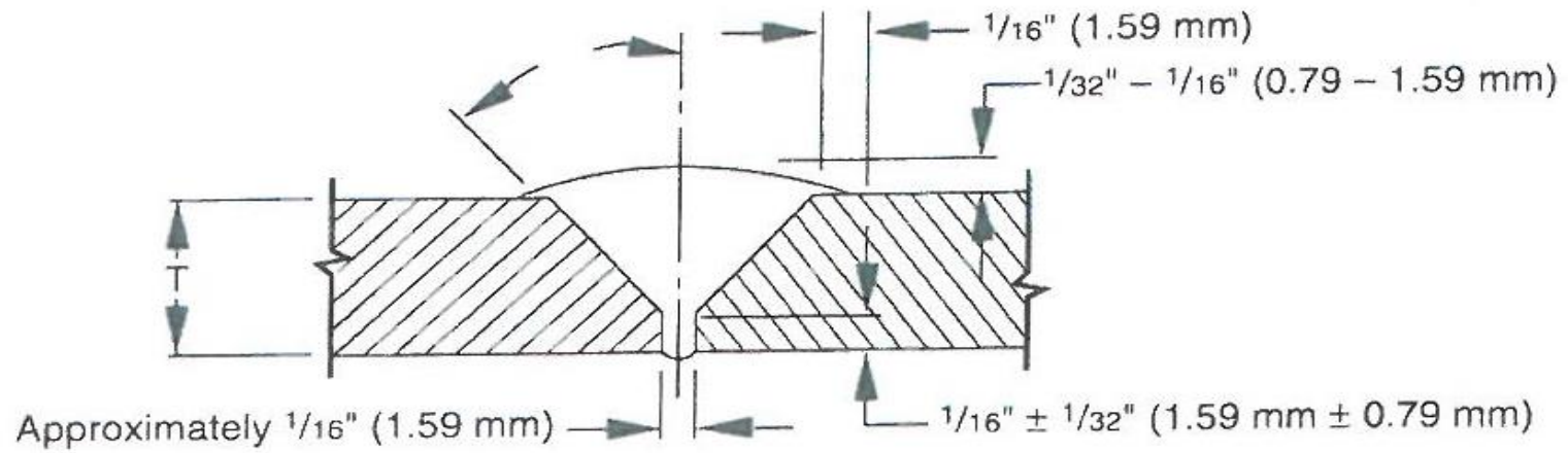
Standard V-Bevel Butt Joint
