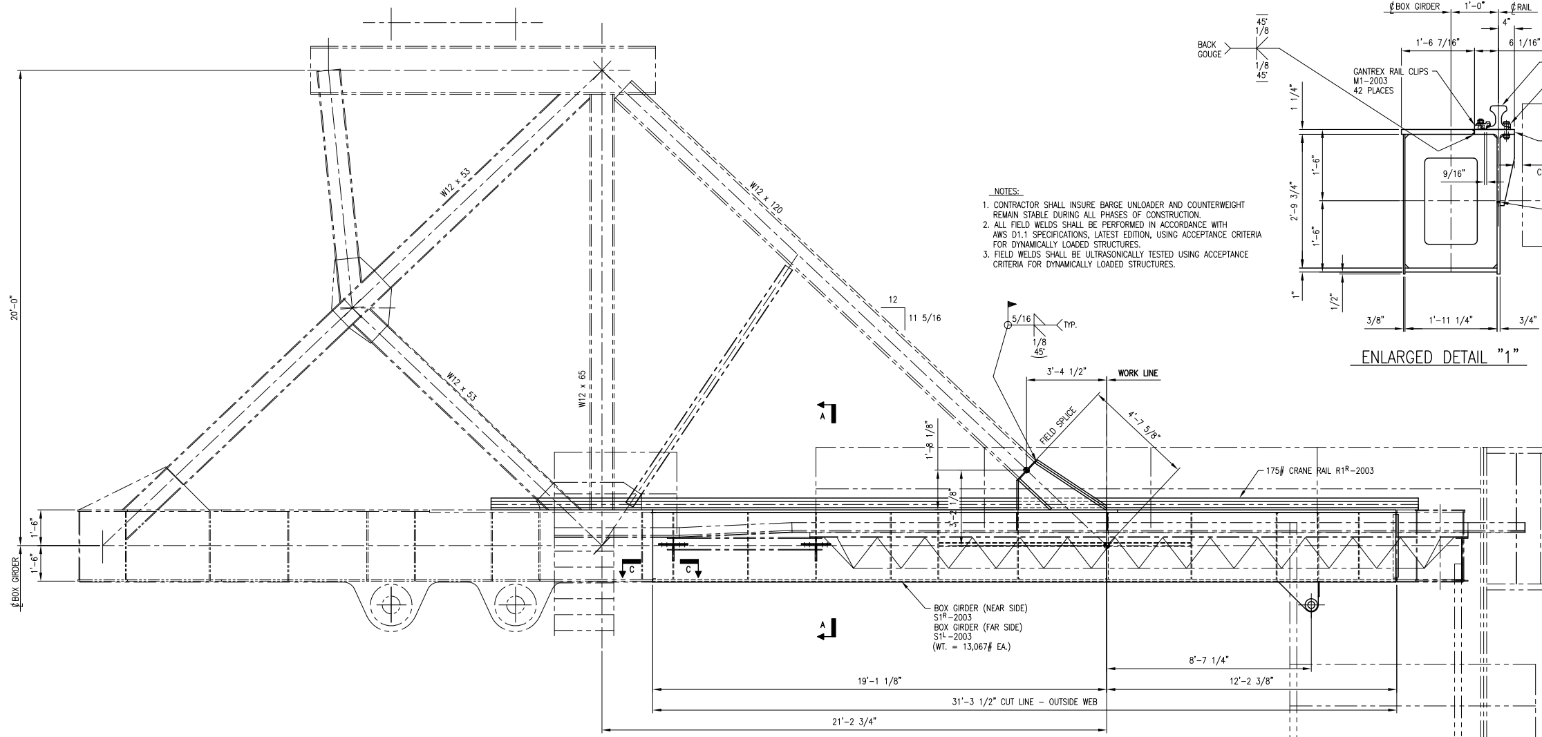
ELEVATION VIEW ~ UNLOADER CANTILEVER SECTION BOX GIRDER REPAIR
