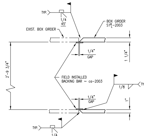
SECTION B-B TYP. 4 PLACES
