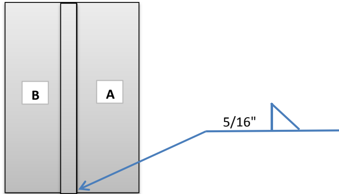
TEE-JOINT 3F UPHILL
