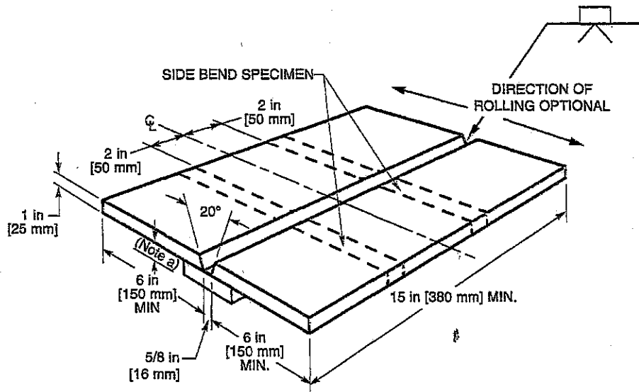
Figure 4.21—Test Plate for Unlimited Thickness—Welder Qualification (see 4.23.1)
