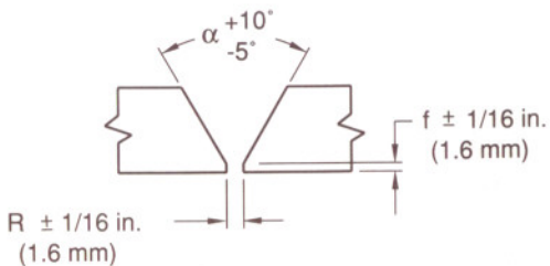
(A) GROOVE WELD WITHOUT BACKING - ROOT NOT BACKGOUGED
