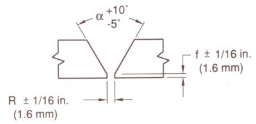
(A) GROOVE WELD WITHOUT BACKING - ROOT NOT BACKGOUGED
